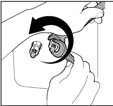
Fig. 14: Removing adapter
